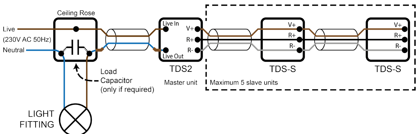
Figure 6 Typical ceiling rose plan using two TDS-S slave units
